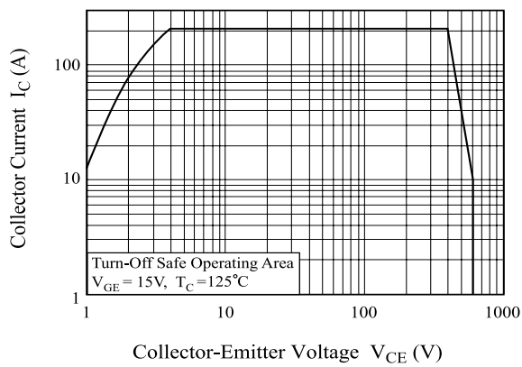
Fig 18. Turn-Off SOA
