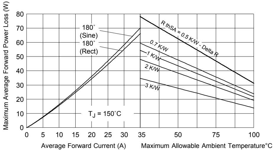
Fig. 3 - Total Power Loss Characteristics
